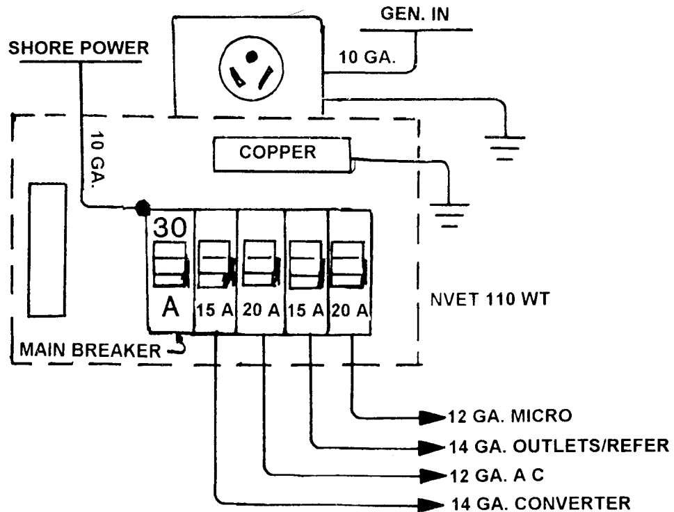
110 VAC BREAKER PANEL DIAGRAM PREMIER ONLY
